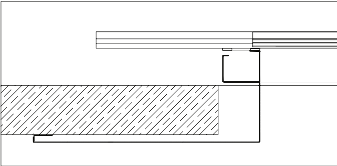
Horizontal section: landing door with door frame / stainless steel portal.
